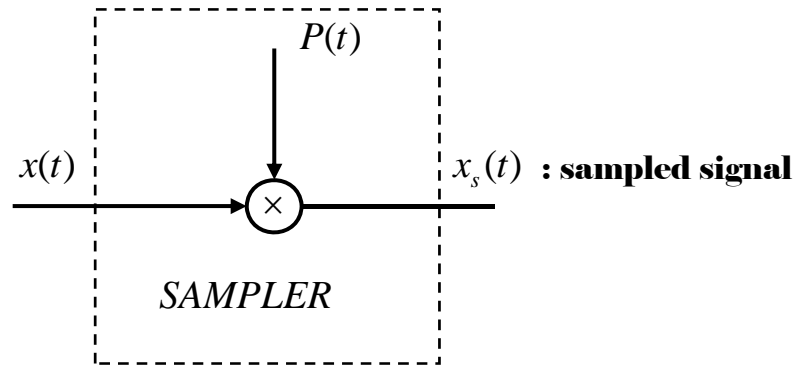
Block diagram
